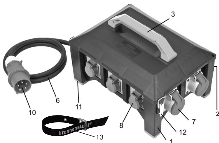
Fig. A, ex. Distribution box BSV 5 3/6 N560
